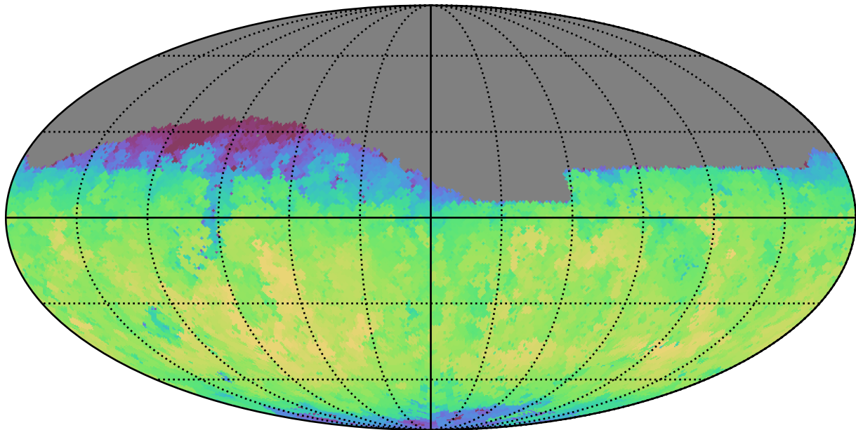
weather_cloudso6v3.4_10yrs Yr 1 i band: Max fiveSigmaDepth
