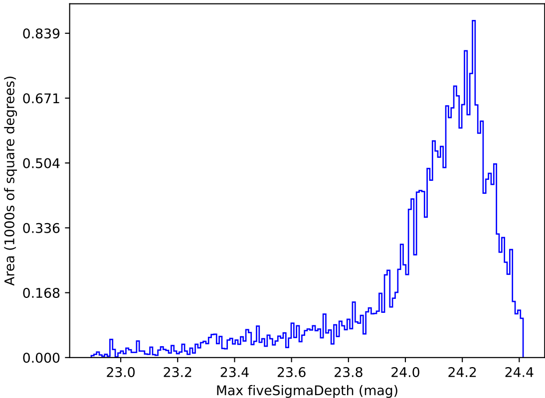
weather_cloudso6v3.4_10yrs Yr 1 i band: Max fiveSigmaDepth
