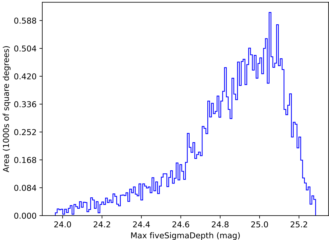
weather_cloudso6v3.4_10yrs Yr 1 g band: Max fiveSigmaDepth
