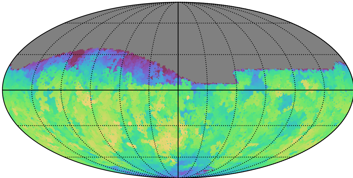
weather_cloudso6v3.4_10yrs Yr 1 all bands: Max fiveSigmaDepth
