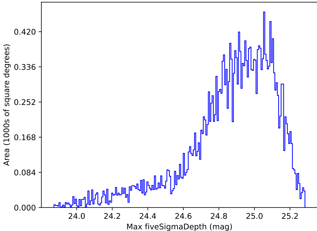
weather_cloudso6v3.4_10yrs Yr 1 all bands: Max fiveSigmaDepth
