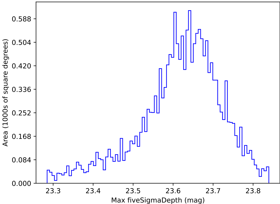
weather_cloudso6v3.4_10yrs WFD z band: Max fiveSigmaDepth
