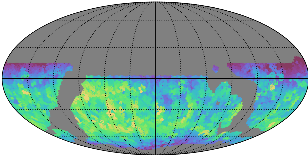
weather_cloudso6v3.4_10yrs WFD r band: Max fiveSigmaDepth
