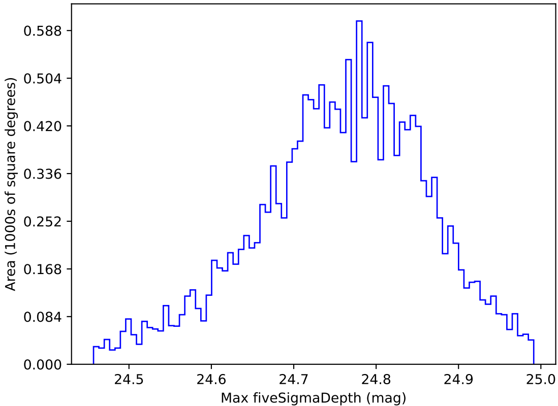
weather_cloudso6v3.4_10yrs WFD r band: Max fiveSigmaDepth
