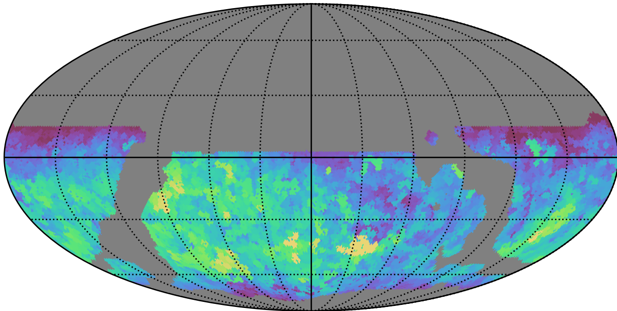
weather_cloudso6v3.4_10yrs WFD g band: Max fiveSigmaDepth
