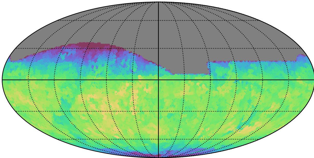
weather_cloudso6v3.4_10yrs All sky z band: Max fiveSigmaDepth
