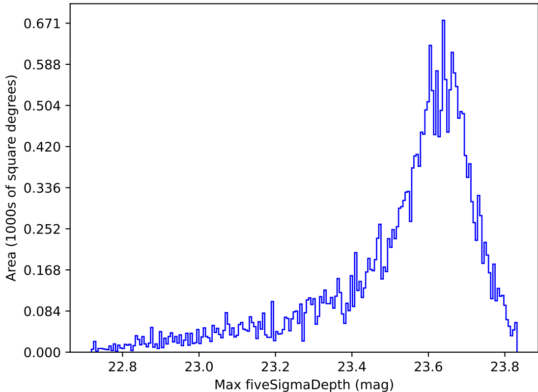
weather_cloudso6v3.4_10yrs All sky z band: Max fiveSigmaDepth
