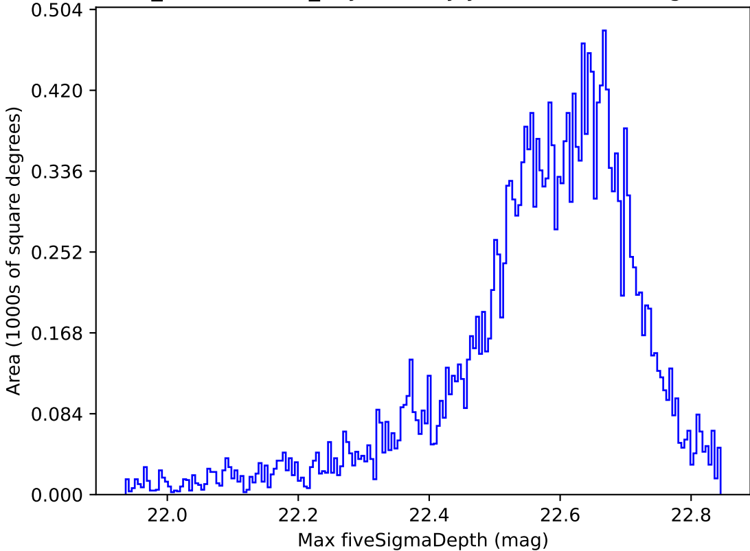
weather_cloudso6v3.4_10yrs All sky y band: Max fiveSigmaDepth
