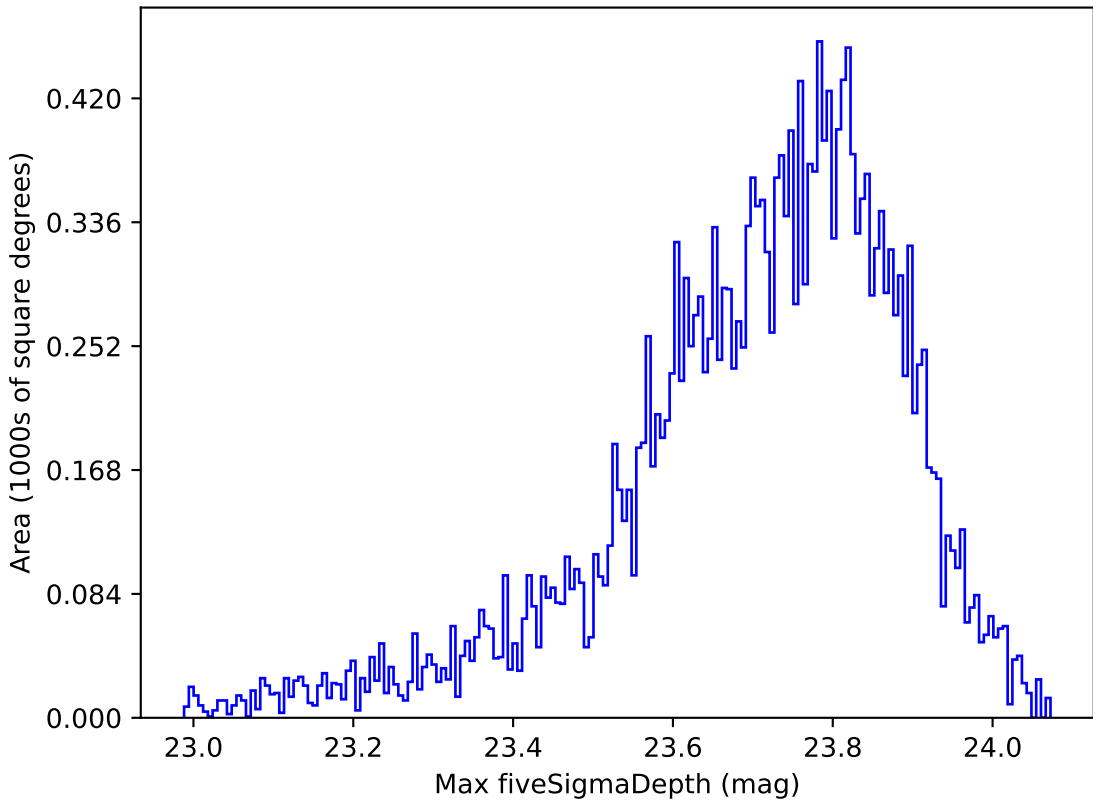
weather_cloudso6v3.4_10yrs All sky u band: Max fiveSigmaDepth
