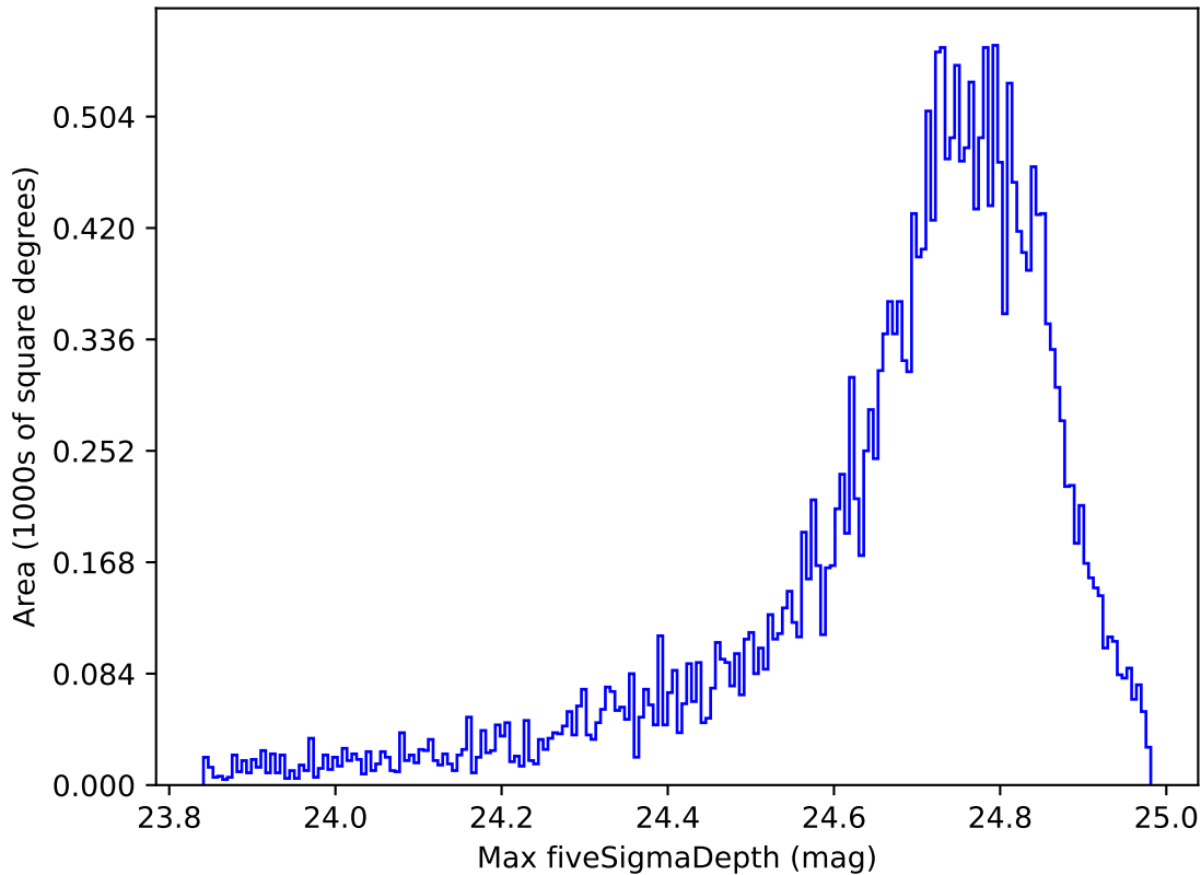
weather_cloudso6v3.4_10yrs All sky r band: Max fiveSigmaDepth
