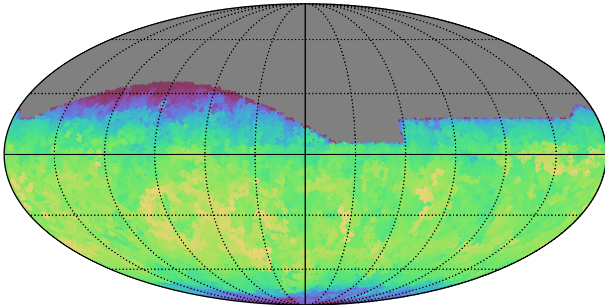
weather_cloudso6v3.4_10yrs All sky i band: Max fiveSigmaDepth
