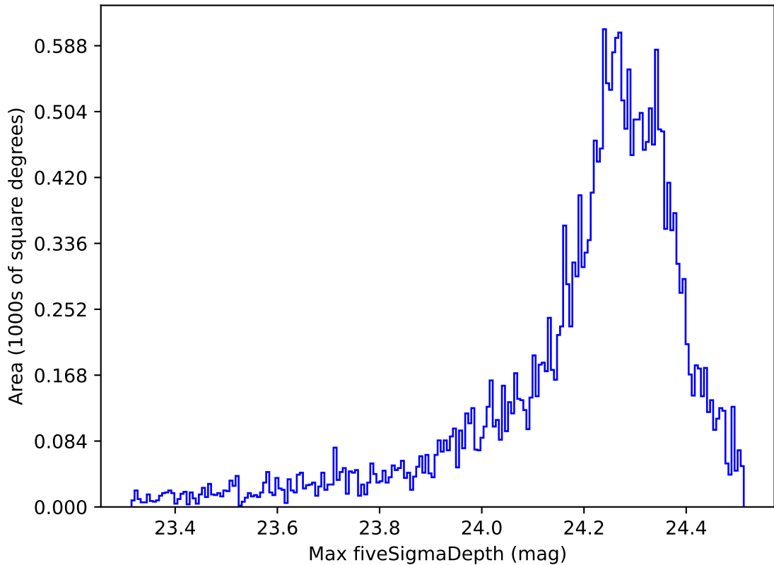
weather_cloudso6v3.4_10yrs All sky i band: Max fiveSigmaDepth
