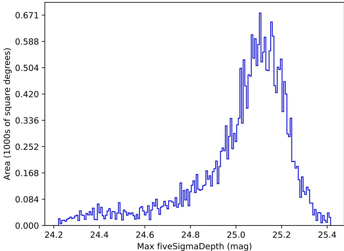
weather_cloudso6v3.4_10yrs All sky g band: Max fiveSigmaDepth
