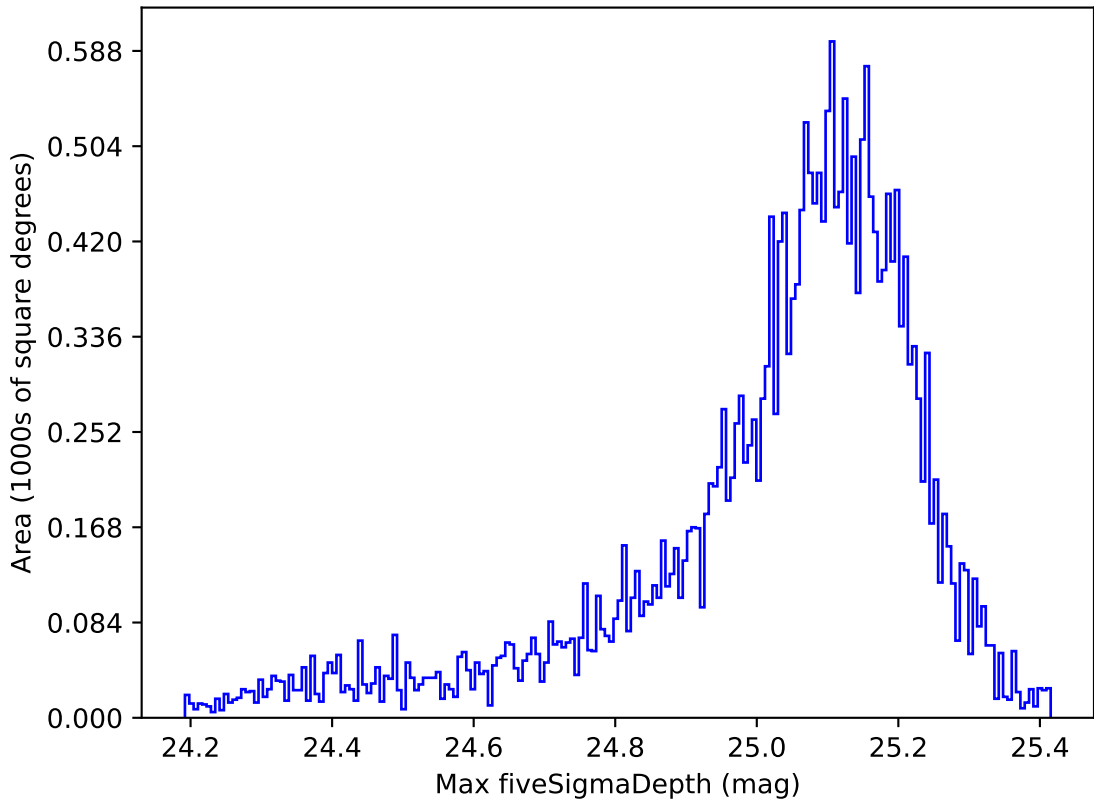
weather_cloudso6v3.4_10yrs All sky all bands: Max fiveSigmaDepth
