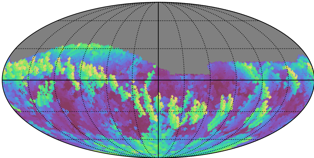
weather_cloudso6v3.4_10yrs Yr 1 z band: Max airmass
