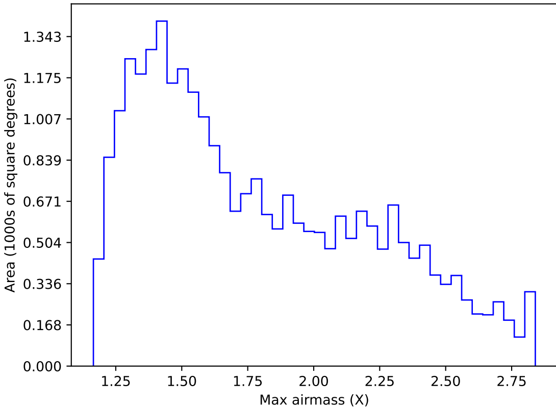
weather_cloudso6v3.4_10yrs Yr 1 z band: Max airmass
