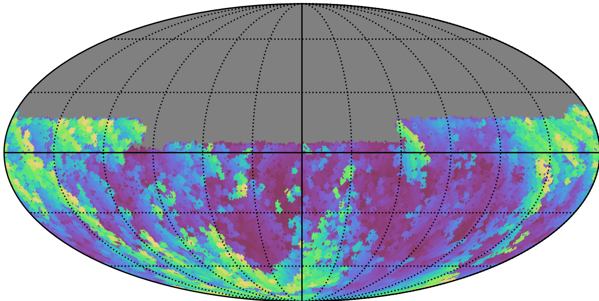
weather_cloudso6v3.4_10yrs Yr 1 y band: Max airmass
