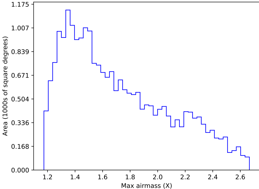
weather_cloudso6v3.4_10yrs Yr 1 y band: Max airmass
