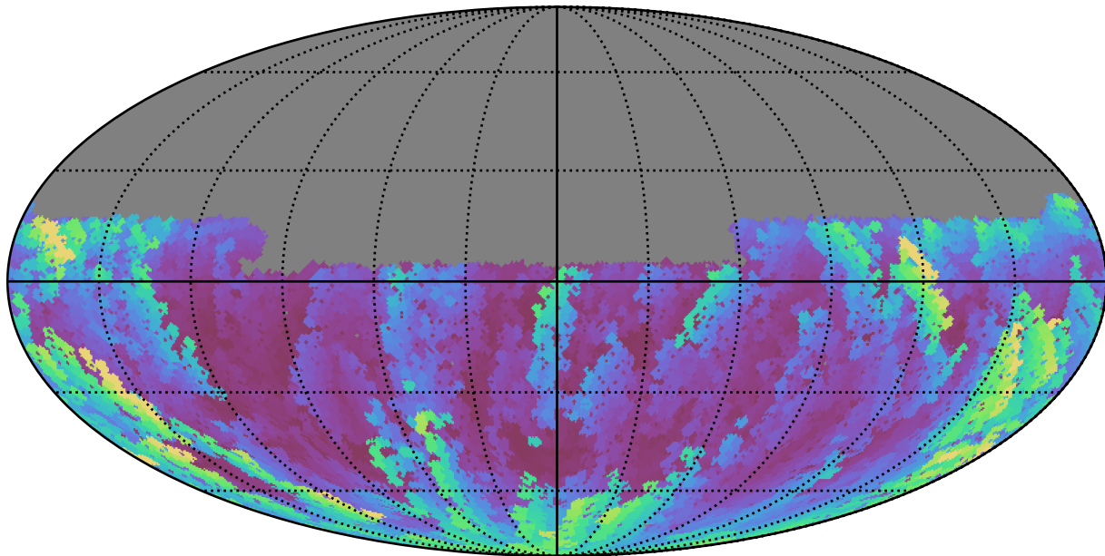
weather_cloudso6v3.4_10yrs Yr 1 u band: Max airmass
