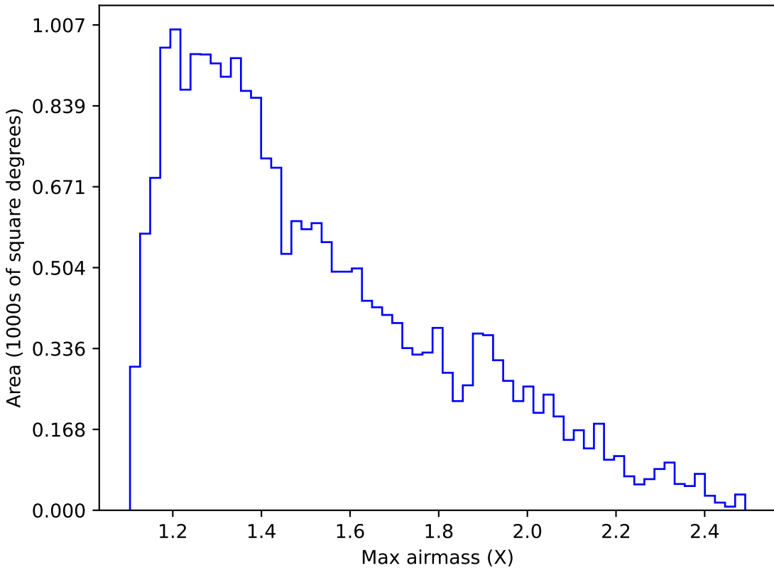
weather_cloudso6v3.4_10yrs Yr 1 u band: Max airmass
