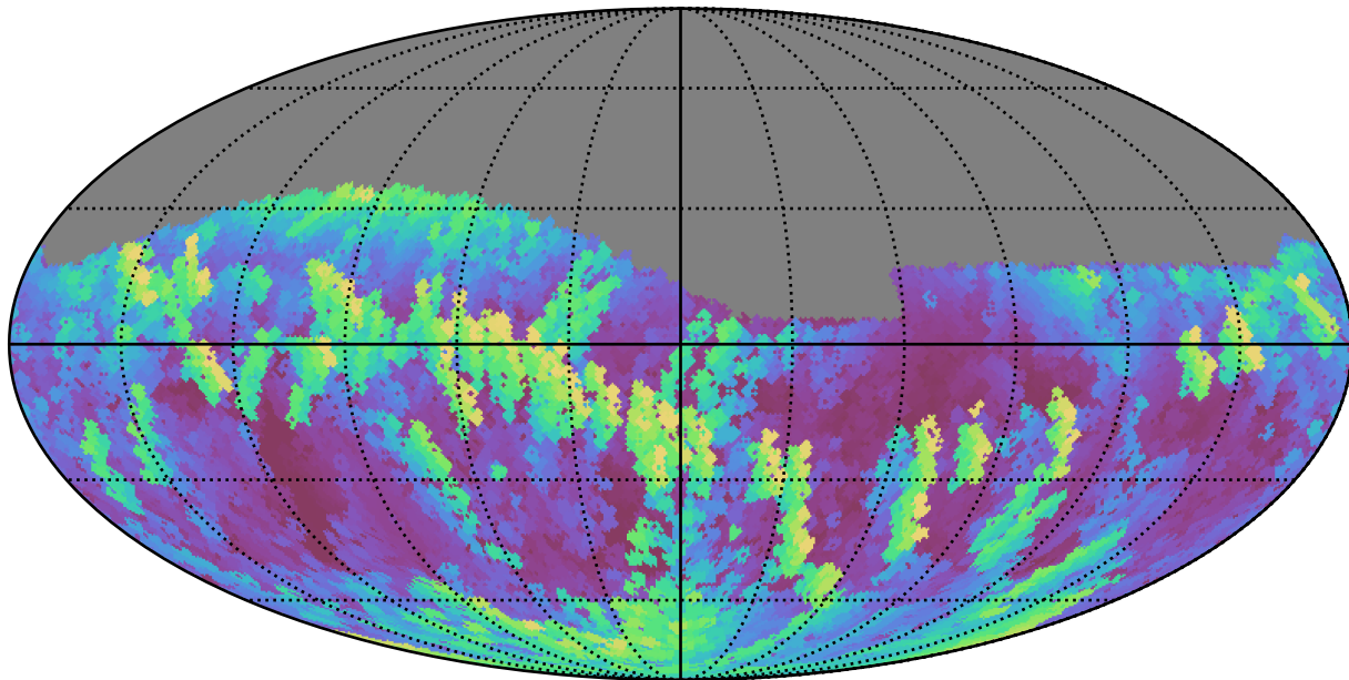
weather_cloudso6v3.4_10yrs Yr 1 i band: Max airmass
