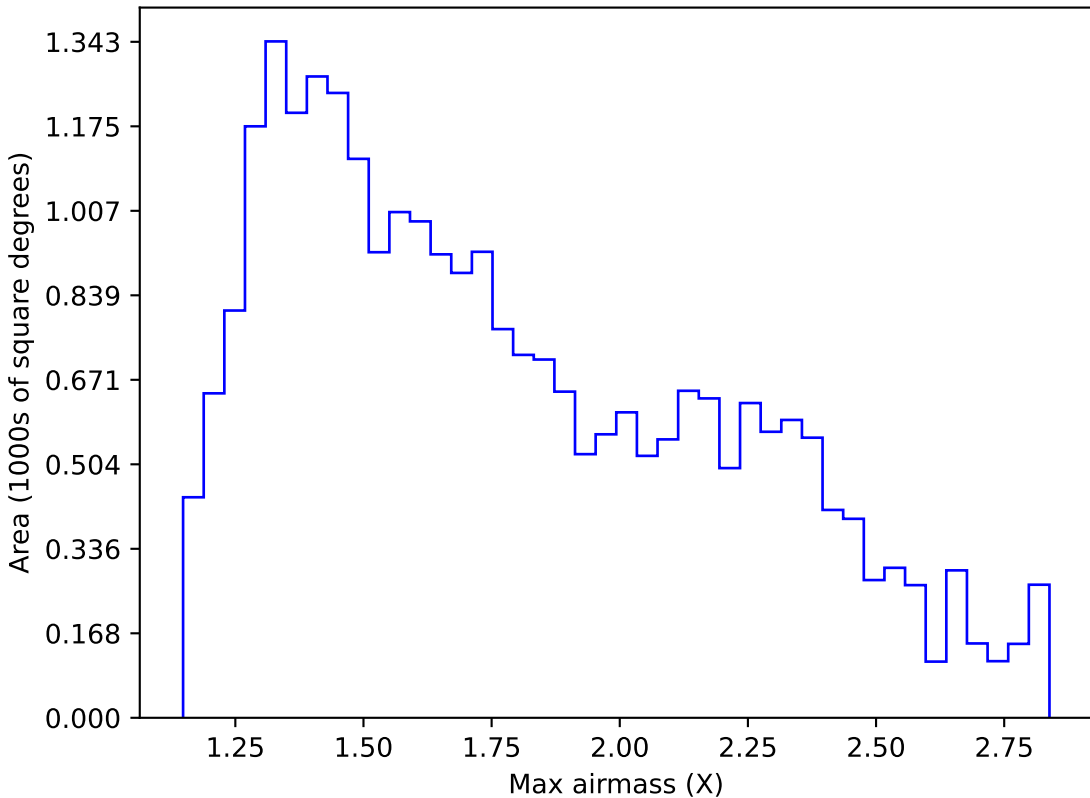
weather_cloudso6v3.4_10yrs Yr 1 i band: Max airmass
