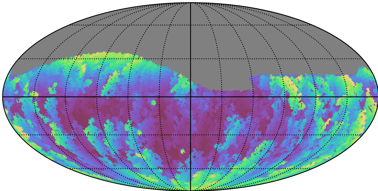
weather_cloudso6v3.4_10yrs Yr 1 g band: Max airmass
