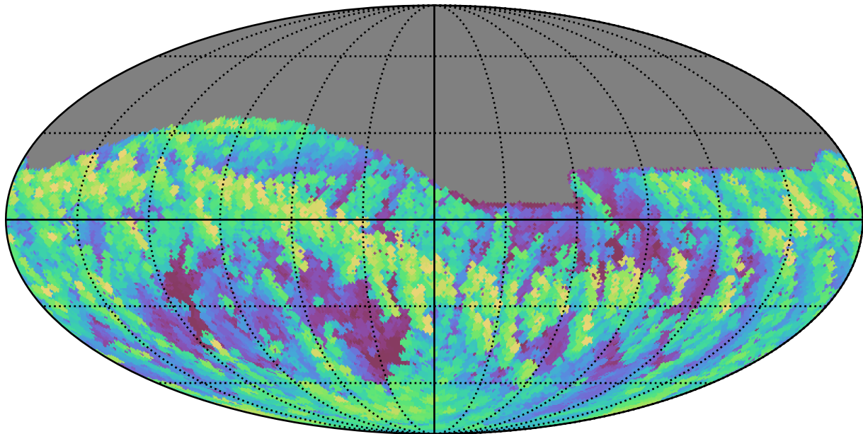
weather_cloudso6v3.4_10yrs Yr 1 all bands: Max airmass
