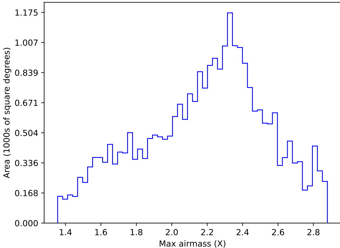
weather_cloudso6v3.4_10yrs Yr 1 all bands: Max airmass
