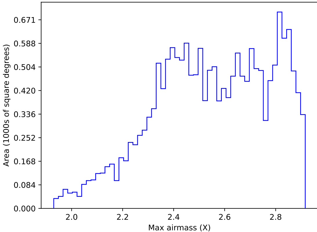
weather_cloudso6v3.4_10yrs WFD z band: Max airmass
