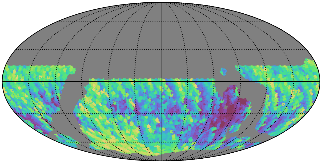
weather_cloudso6v3.4_10yrs WFD y band: Max airmass
