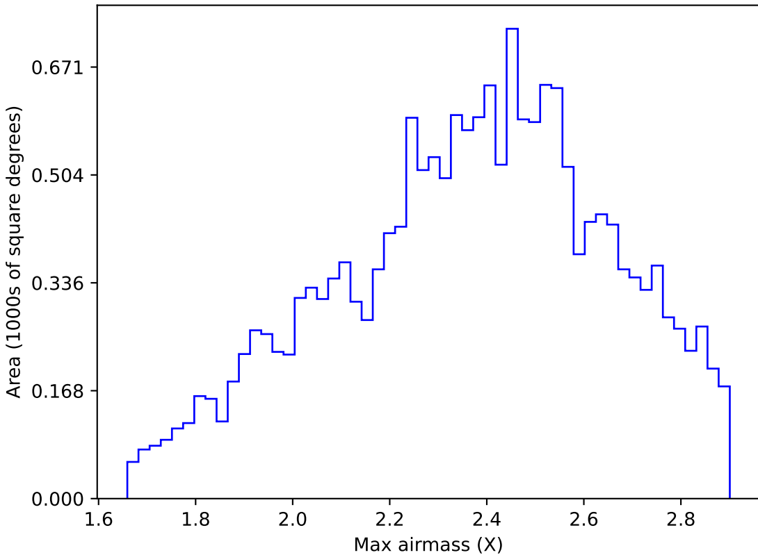
weather_cloudso6v3.4_10yrs WFD y band: Max airmass
