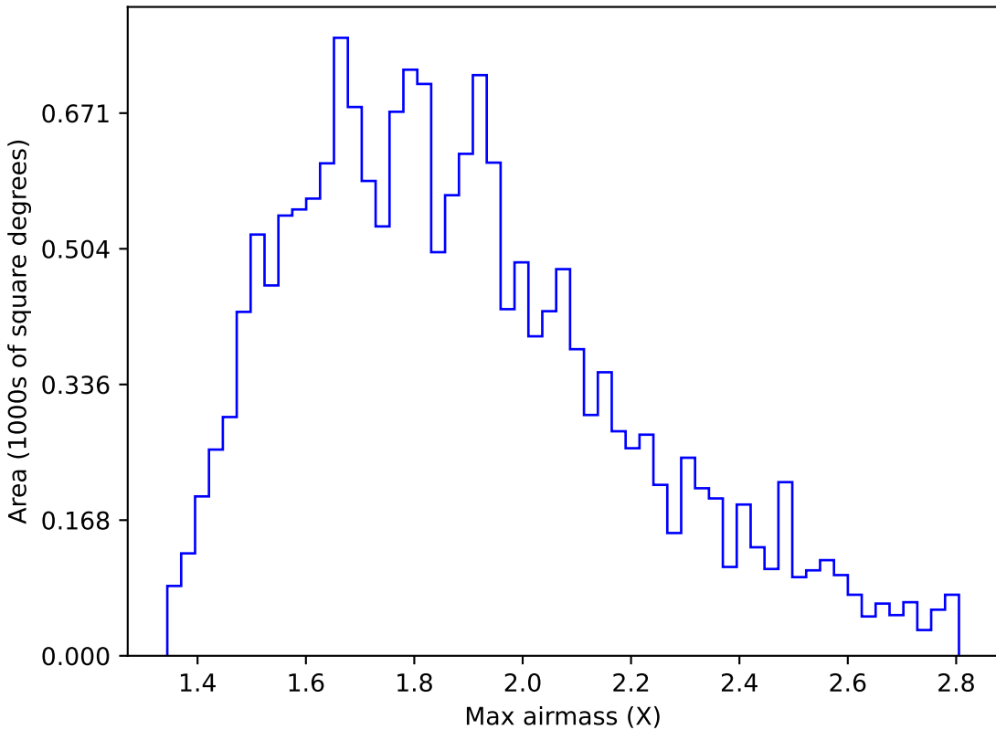
weather_cloudso6v3.4_10yrs WFD u band: Max airmass
