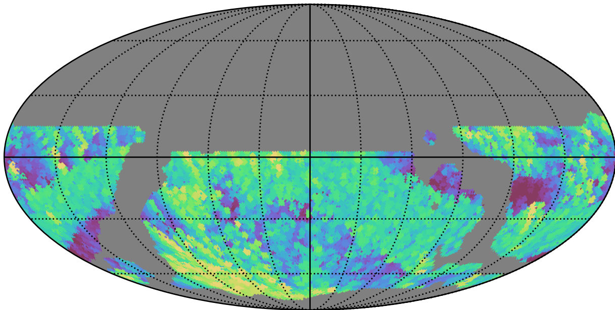
weather_cloudso6v3.4_10yrs WFD r band: Max airmass
