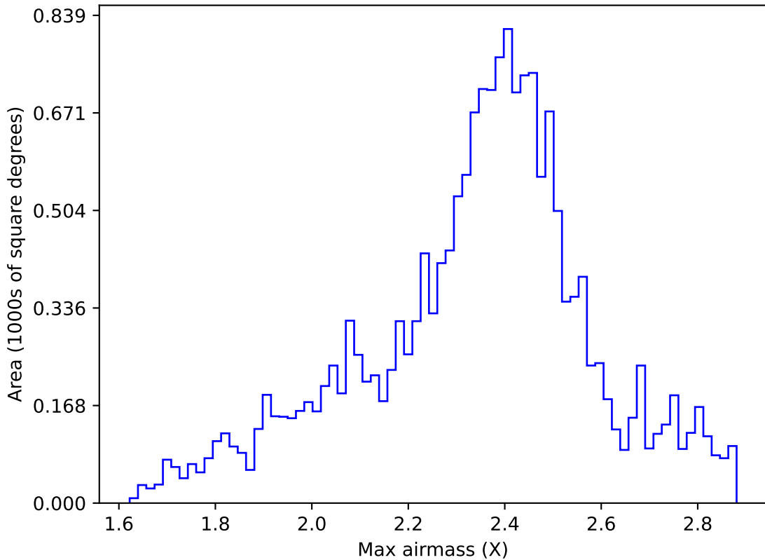
weather_cloudso6v3.4_10yrs WFD r band: Max airmass
