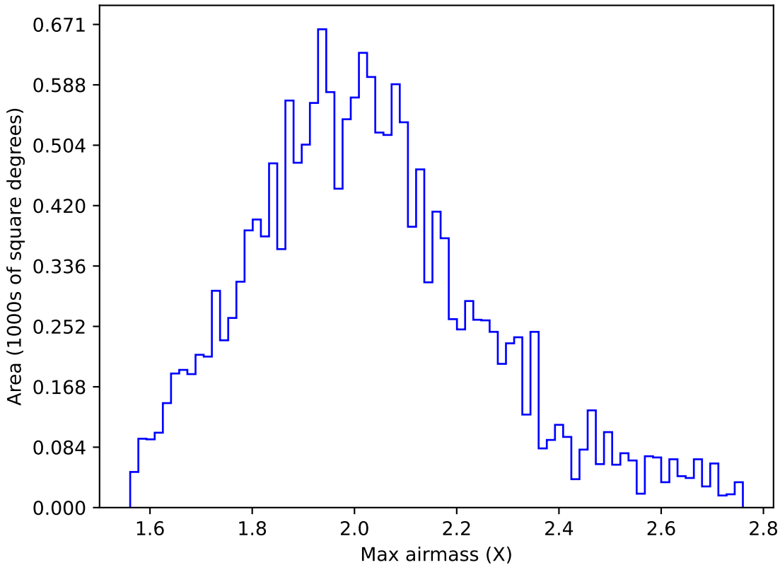
weather_cloudso6v3.4_10yrs WFD g band: Max airmass
