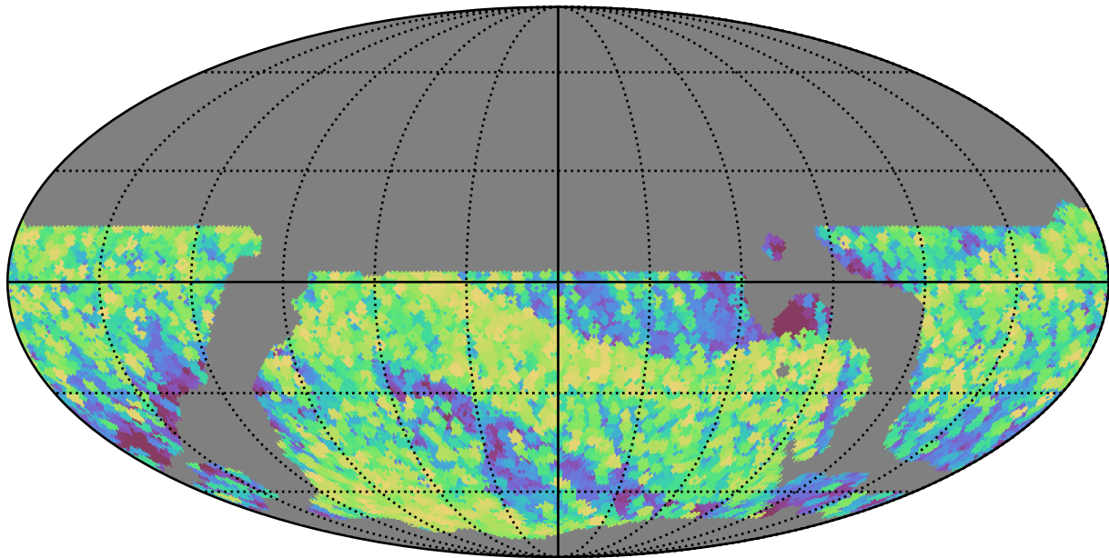
weather_cloudso6v3.4_10yrs WFD all bands: Max airmass
