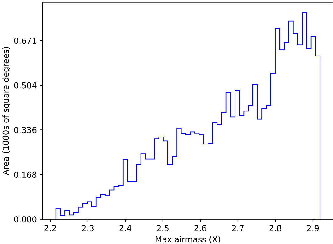
weather_cloudso6v3.4_10yrs WFD all bands: Max airmass
