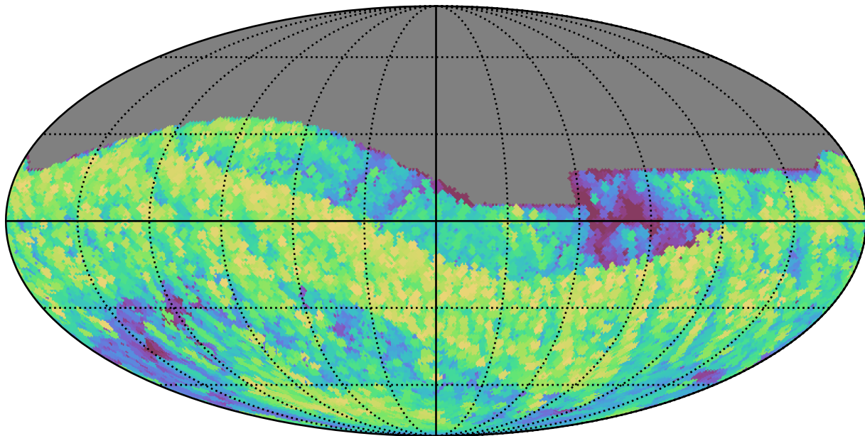
weather_cloudso6v3.4_10yrs All sky z band: Max airmass
