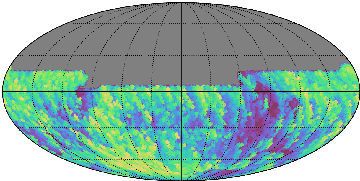
weather_cloudso6v3.4_10yrs All sky y band: Max airmass
