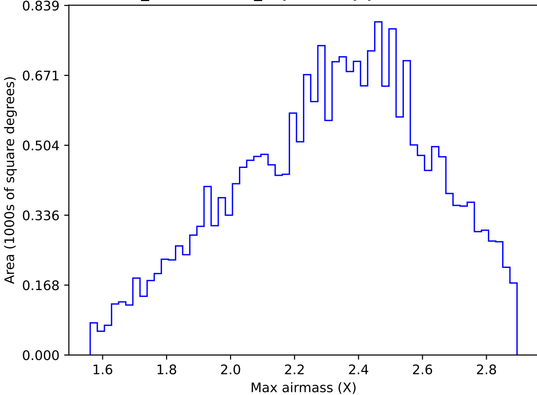
weather_cloudso6v3.4_10yrs All sky y band: Max airmass
