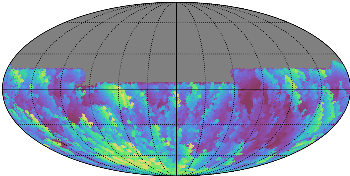
weather_cloudso6v3.4_10yrs All sky u band: Max airmass
