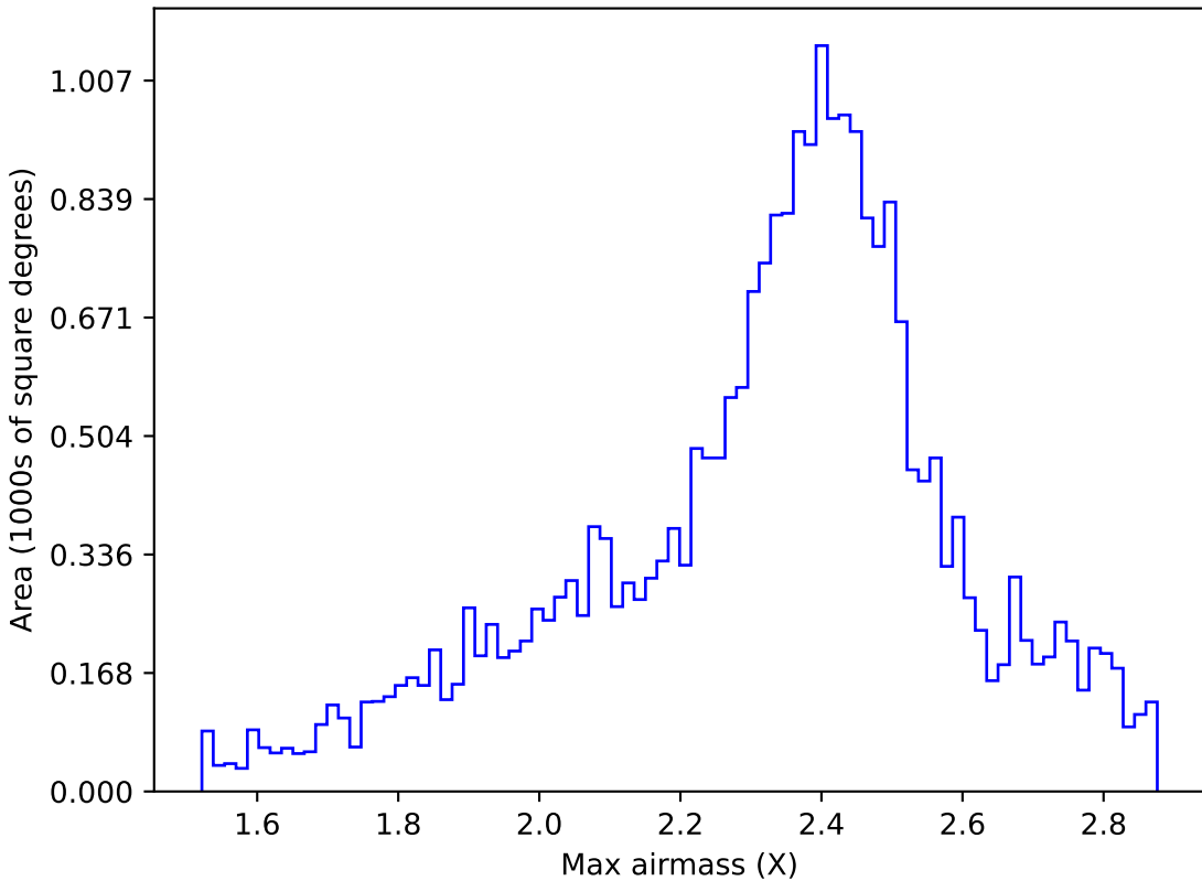
weather_cloudso6v3.4_10yrs All sky r band: Max airmass
