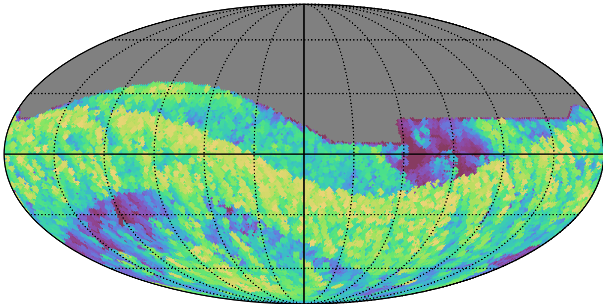
weather_cloudso6v3.4_10yrs All sky i band: Max airmass
