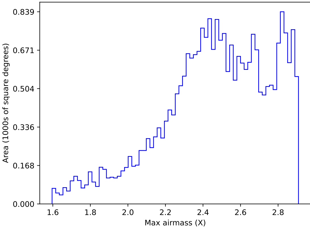
weather_cloudso6v3.4_10yrs All sky i band: Max airmass
