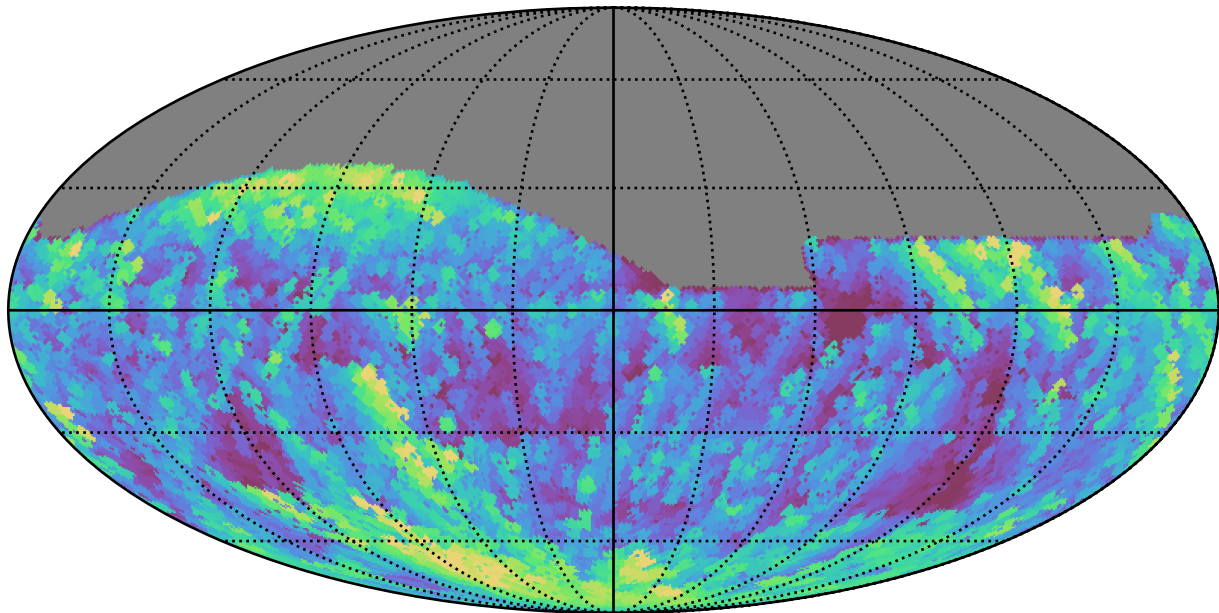
weather_cloudso6v3.4_10yrs All sky g band: Max airmass
