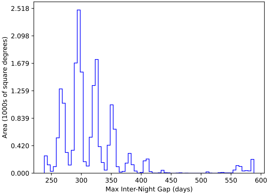
weather_cloudso6v3.4_10yrs WFD y band: Max Inter-Night Gap
