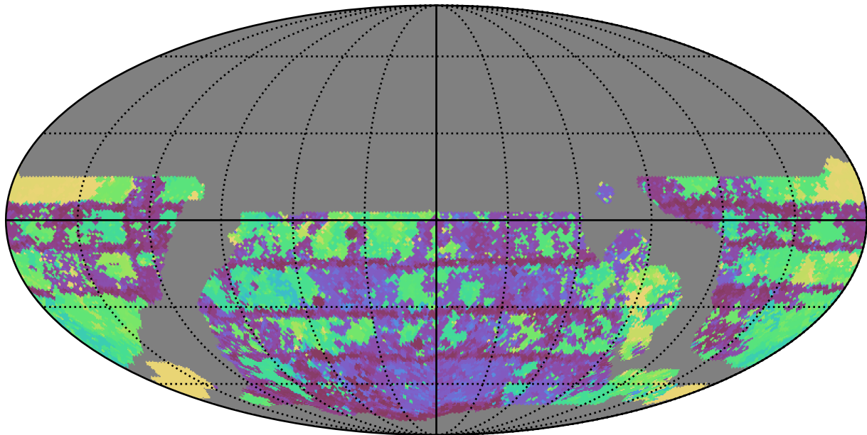
weather_cloudso6v3.4_10yrs WFD u band: Max Inter-Night Gap
