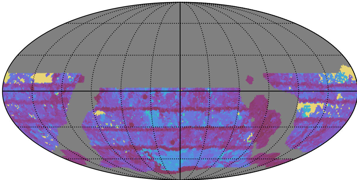
weather_cloudso6v3.4_10yrs WFD r band: Max Inter-Night Gap
