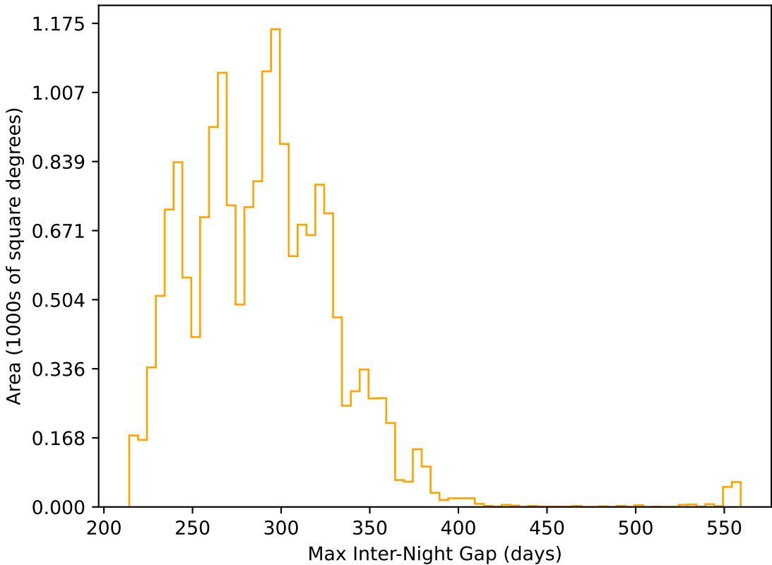
weather_cloudso6v3.4_10yrs WFD r band: Max Inter-Night Gap
